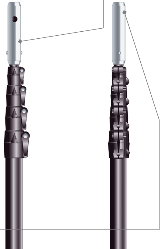
Mechanism of locking by control lever
